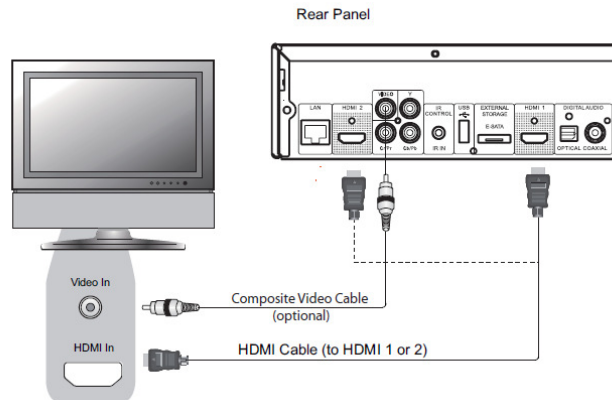
Method 1 – HDMI Connection directly to a single TV
