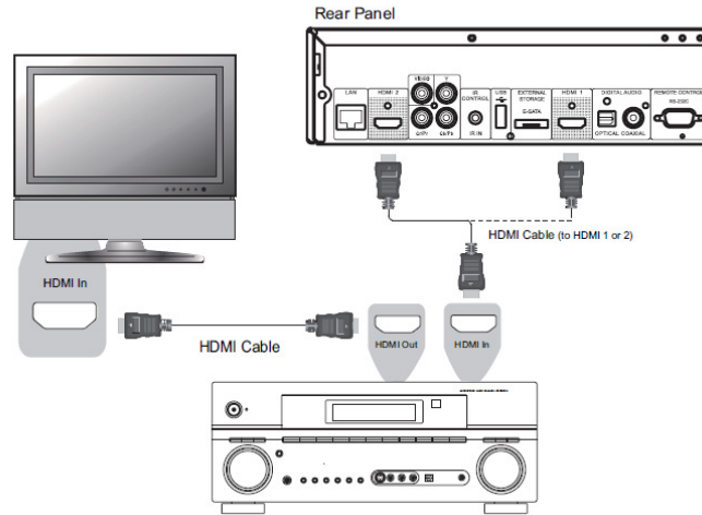
Method 5 – HDMI Connection to Receiver and TV
