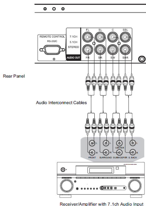
Method 6 – 7.1ch Analog Audio Connection
