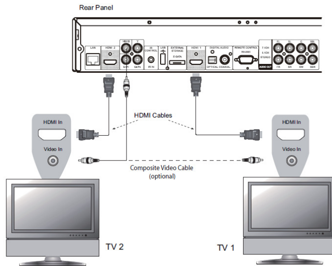
Method 2 – HDMI Connection directly to two TVs
