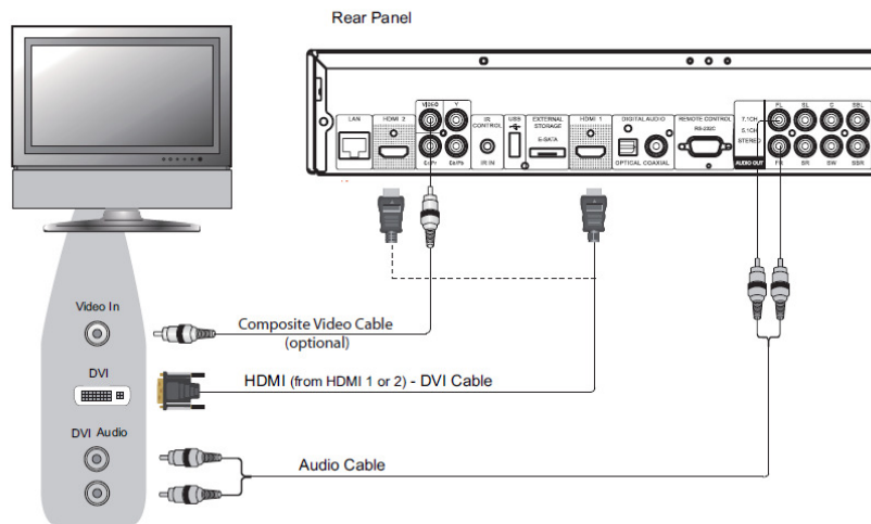
Method 3 – DVI Connection to TV
