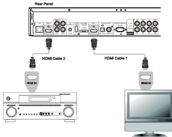
Method 9 – Dual HDMI Connection
