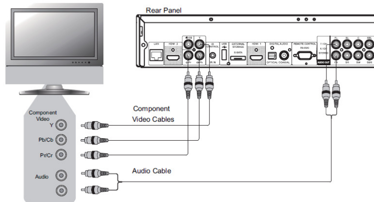
Method 4 – Component Video Connection to TV
